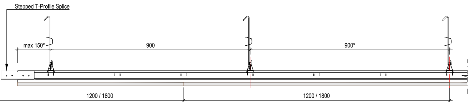
CROSS-SECTION 1 scale 1:10
