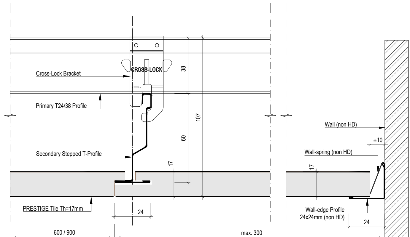
DETAIL SECTION 3 scale 1:1,5
