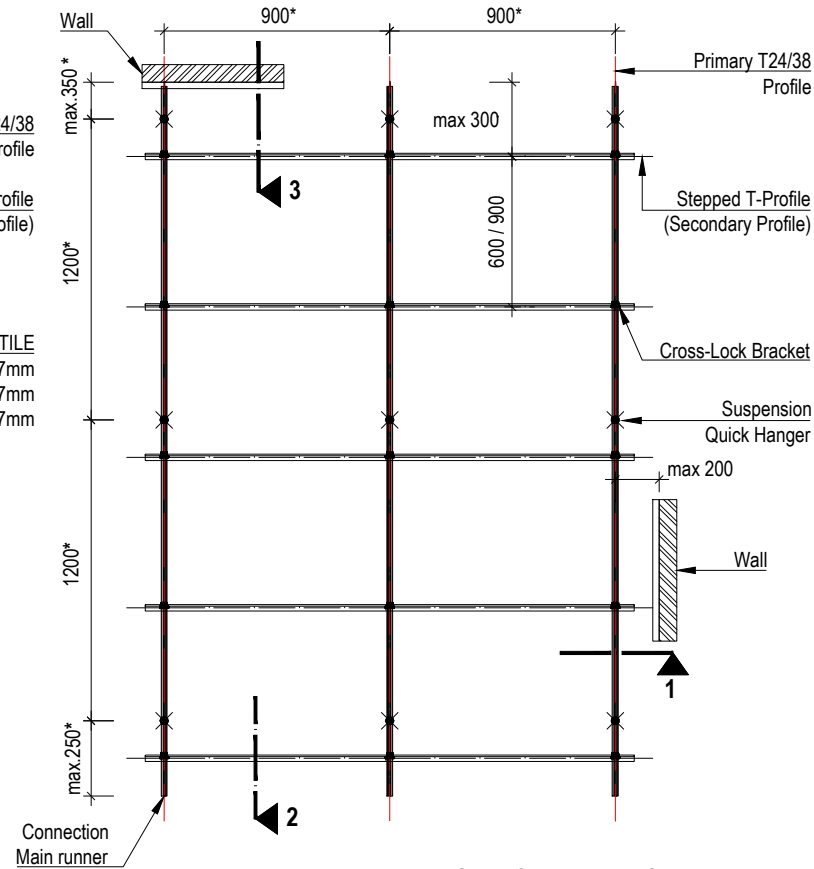
STRUCTURE LAY-OUT scale 1:30
