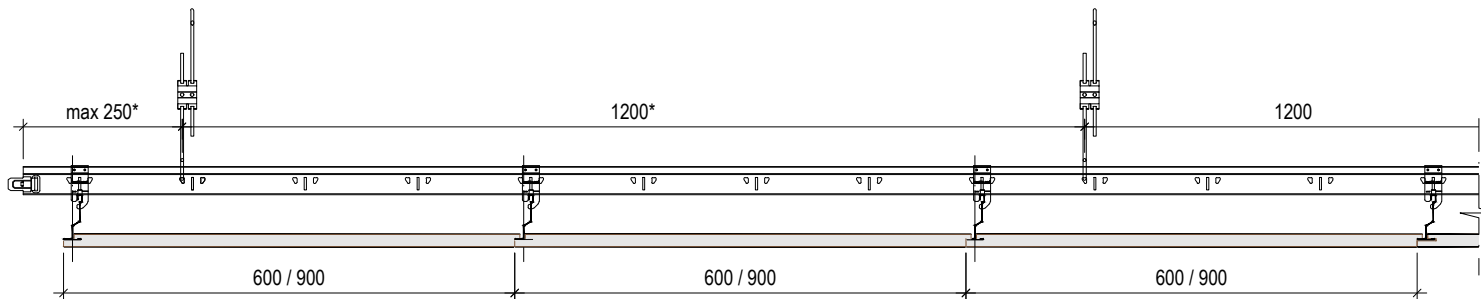
CROSS-SECTION 2 scale 1:10
