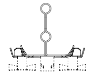
RAIL (FOR MOVABLE PANEL) -front
