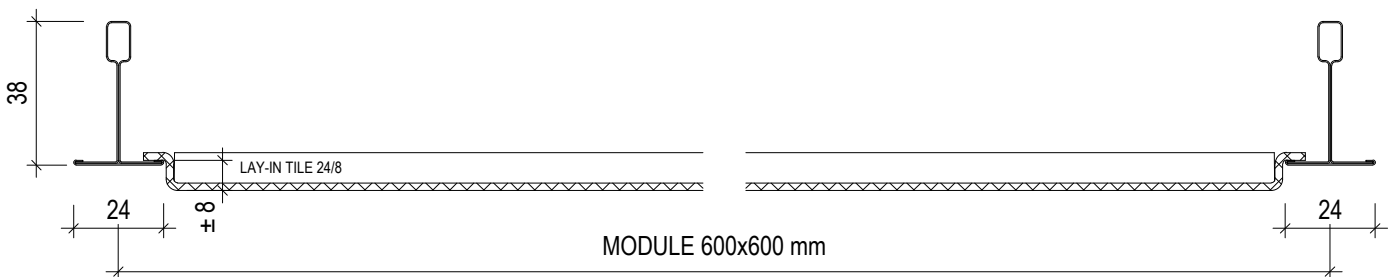
T-PROFILE 38x24 (non HD) side
