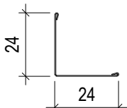
EDGE PROFILE 24X24 mm (non HD) sec
