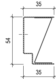
EDGE-PROFILE UW 50 L= max.3000 mm
