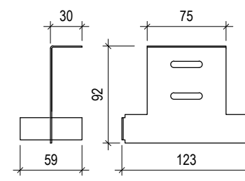
Front view Side-view parallel
