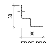
EDGE-PROFILE W 30 L= max.3000 mm
