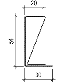
EDGE-PROFILE U 50 L= max.3000 mm
