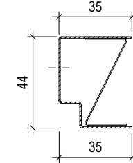
EDGE-PROFILE UW 40 L= max.3000 mm
