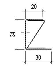
EDGE-PROFILE U 30 L= max.3000 mm
