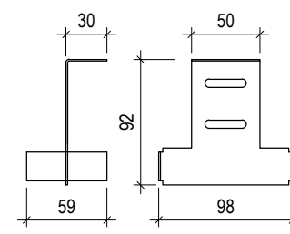
Front view Side-view parallel
