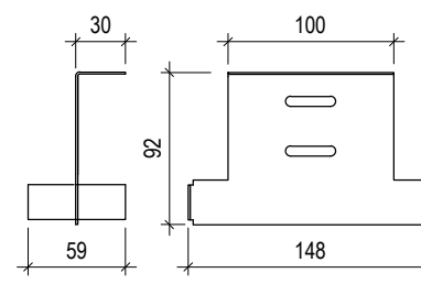
Front view Side-view parallel
