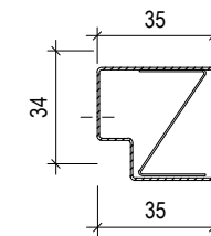
EDGE-PROFILE UW 30 L= max.3000 mm
