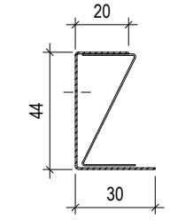
EDGE-PROFILE U 40 L= max.3000 mm
