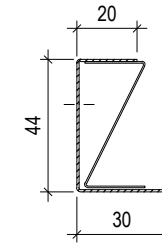
EDGE-PROFILE U 40 L= max.3000 mm
