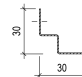
EDGE-PROFILE W 30 L= max.3000 mm
