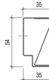
EDGE-PROFILE UW 50 L= max.3000 mm
