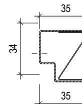
EDGE-PROFILE UW 30 L= max.3000 mm
