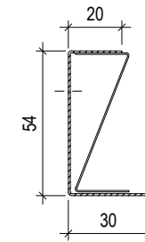
EDGE-PROFILE U 50 L= max.3000 mm
