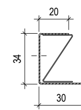
EDGE-PROFILE U 30 L= max.3000 mm
