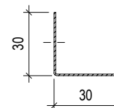
EDGE-PROFILE L 30 L= max.3000 mm
