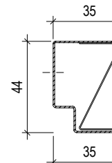
EDGE-PROFILE UW 40 L= max.3000 mm
