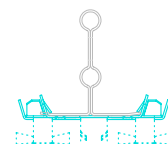
RAIL (FOR MOVABLE PANEL) -front
