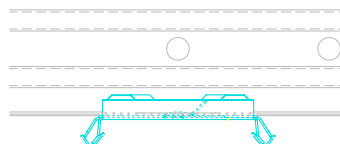
RAIL MOD.89mm. (FOR MOVABLE PANEL) -side
